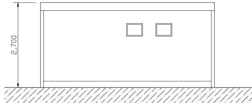
EAST ELEVATION
